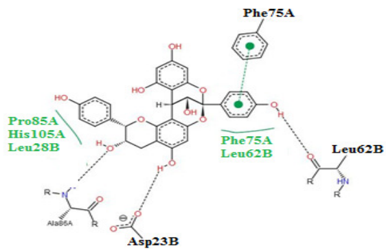
Figure 5. Interactions of compounds with APRT enzyme a) Bryophillin A interactions with APRT, b) Quercetin interactions with APRT, c) Corilagin interactions with APRT, d) Geranin interactions with APRT
