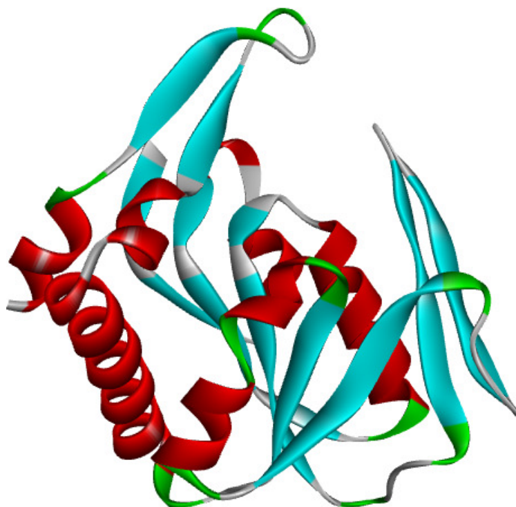
Figure 1. The three dimensional structure of mutated APRT enzyme, the alpha helices are represented by red color while the beta strands are represented by blue color, the grey color represents coil and green color represents turns between strands and coils.
