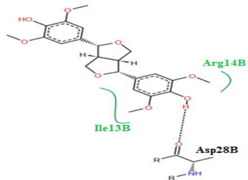
Figure 4. Interactions of compounds with APRT enzyme a) Berberine interactions with APRT, b) Scopoletin interactions with APRT, c) Asiactoside interactions with APRT, d) Syrenegaresinol interactions with APRT
