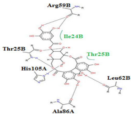
Figure 5. Interactions of compounds with APRT enzyme a) Bryophillin A interactions with APRT, b) Quercetin interactions with APRT, c) Corilagin interactions with APRT, d) Geranin interactions with APRT
