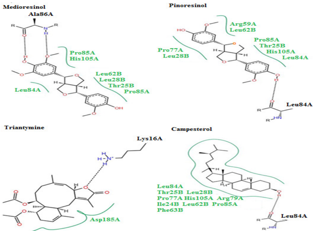
Figure 3. Interactions of compounds with APRT enzyme a) Medioresinol interactions with APRT, b) Pinoresinol interactions with APRT, c) Triantymine interactions with APRT, d) Campesterol interactions with APRT
