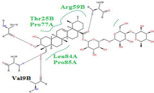
Figure 4. Interactions of compounds with APRT enzyme a) Berberine interactions with APRT, b) Scopoletin interactions with APRT, c) Asiactoside interactions with APRT, d) Syrenegaresinol interactions with APRT
