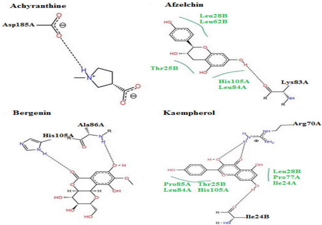
Figure 2. Interactions of compounds with APRT enzyme a) Achyranthine interactions with APRT, b) Afzelchin interactions with APRT, c) Bergenin interactions with APRT, d) Kaempherol interactions with APRT
