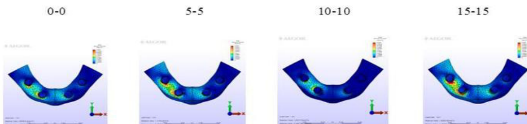
Figure 12. Stresses occurred in right oblique loading
