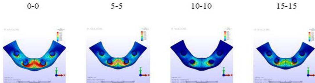
Figure 10. Stresses occurred in anterior oblique loading
