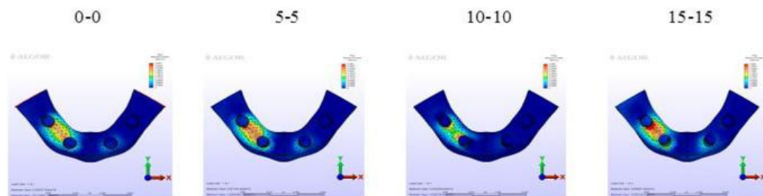
Figure 11. Stresses occurred in right vertical loading
