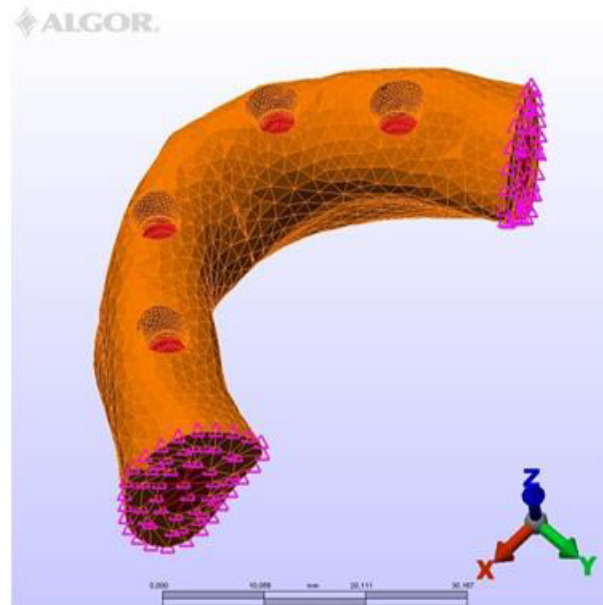
Figure 3. Boundary conditions of the model
