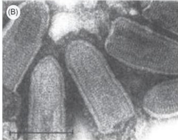
Figure 1. Virus showing characteristic bullet-shaped virions.
